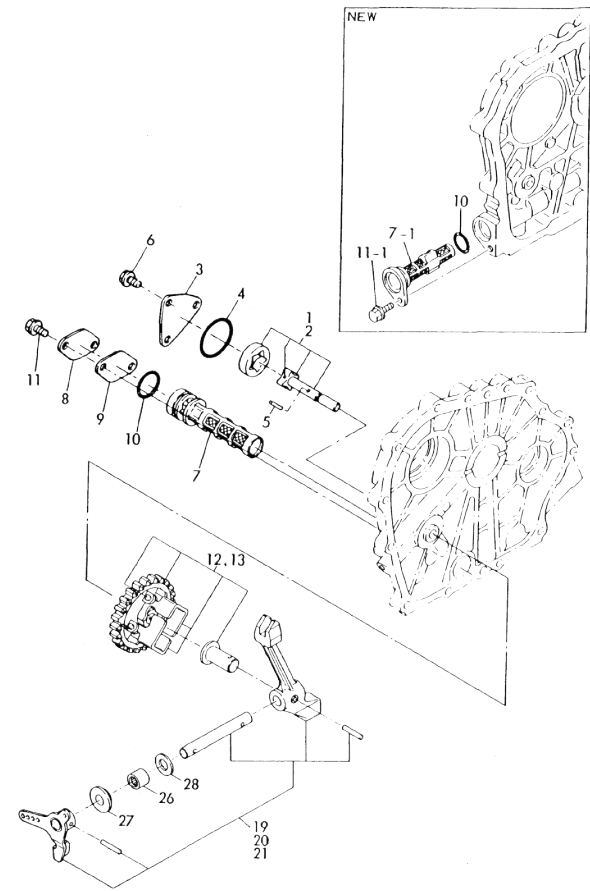
Fig.5 LUB. OIL & GOVERNOR
